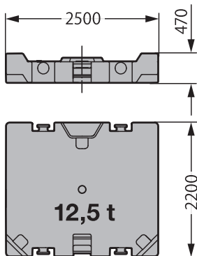
部材C
